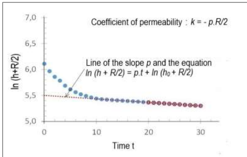
Figure 7. Permeability curve [8]
