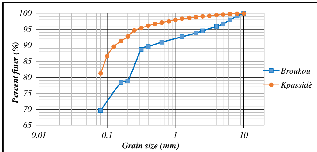
Figure 2. Particle size curves of Broukou and Kpassidè clay soils
