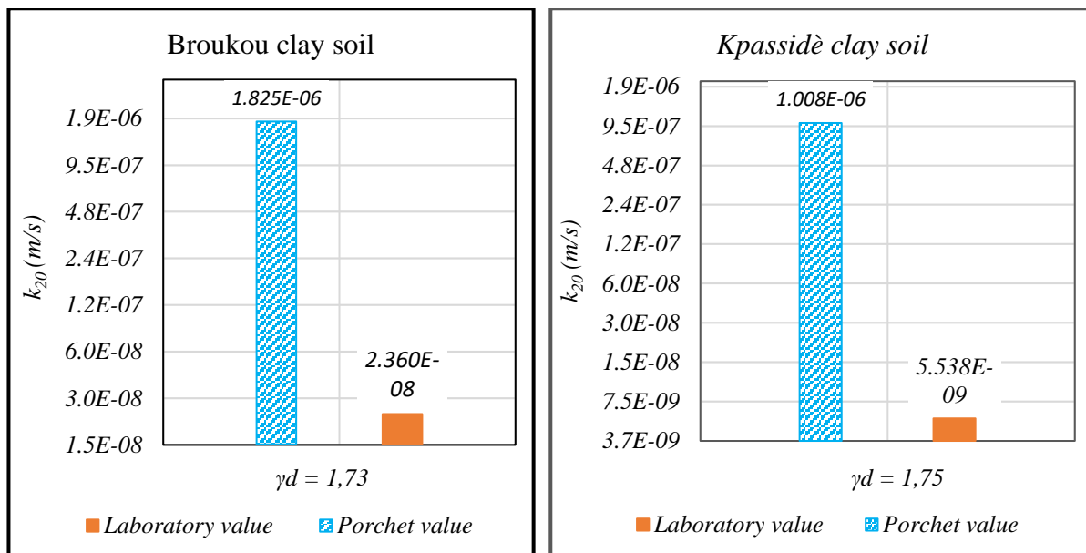
Figure 3. Comparative diagrams of Porchet and variable load permeameter tests results on Broukou and Kpassidè clays soils
