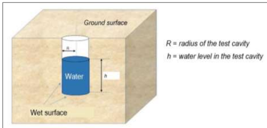
Figure 2. Principle schema of Porchet test [8]
