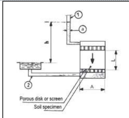
Figure 8. Principle scheme of variable load permeameter [10]
